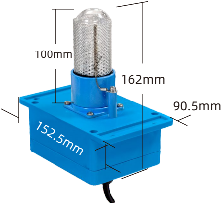
FC-100B (152.5*90.5*162mm)
