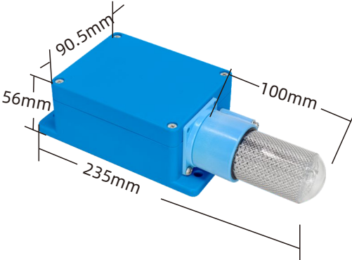
FC-100D (235*90.5*56mm)
