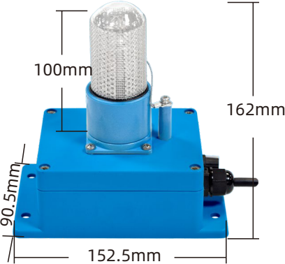
FC-100C (152.5*90.5*162mm)
